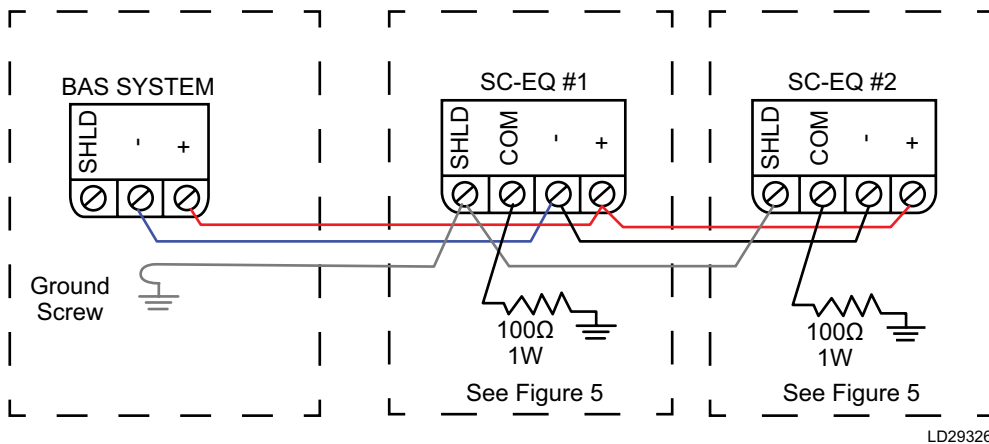
FIGURE 4 - 2-WIRE BAS
