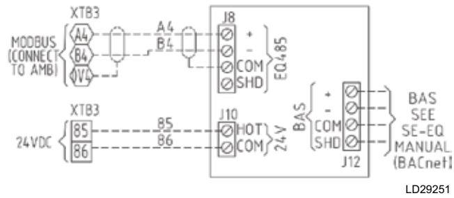
FIGURE 19 - SC-EQ TO YVWE AND YVWH CONNECTIONS
