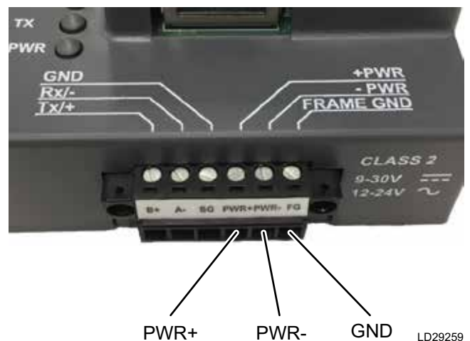
FIGURE 57 - PROTONODE POWER WIRING
