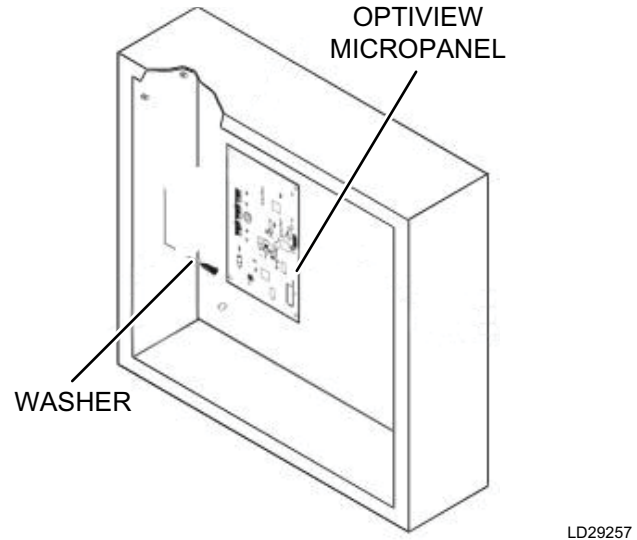
FIGURE 55 - OPTIVIEW LON PROTONODE MOUNTING LOCATION
