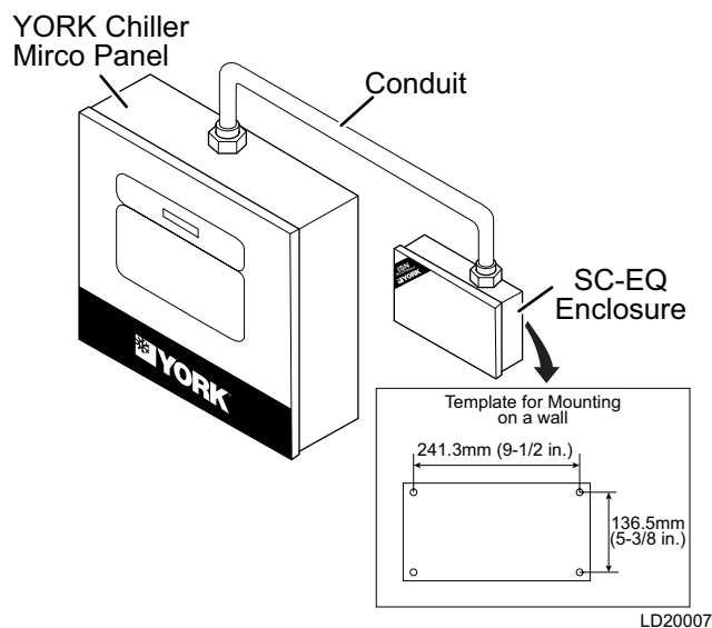
FIGURE 25 - WALL MOUNTING
