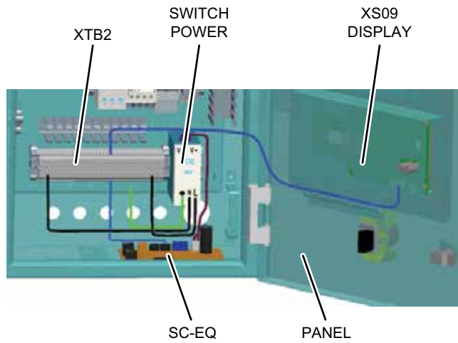
FIGURE 20 - SC-EQ INSTALLED IN YEW S AND YGWE SINGLE
