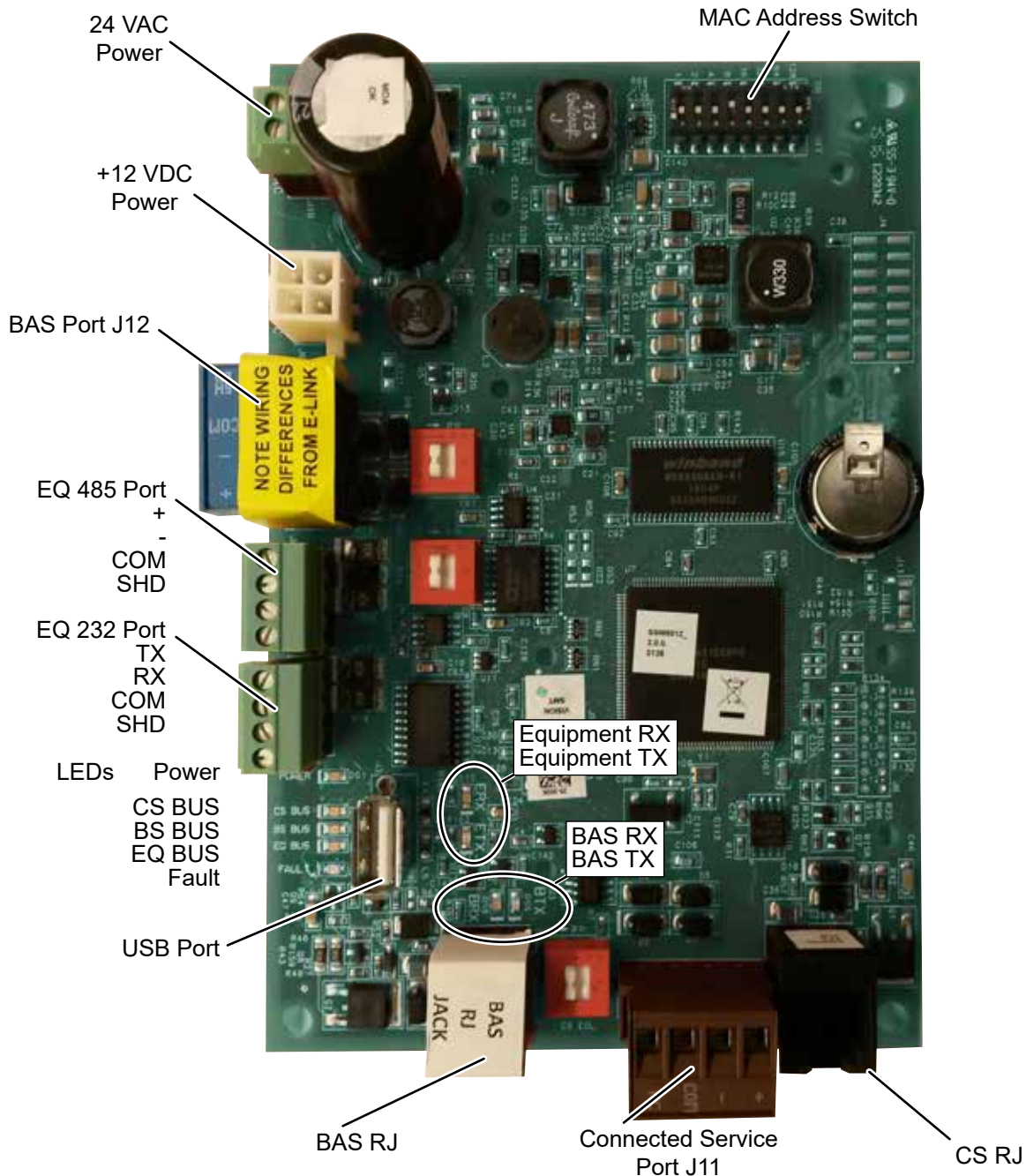
FIGURE 27 - SC-EQ COMPONENT LOCATIONS
