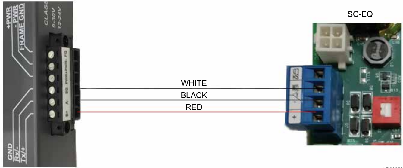
FIGURE 56 - PROTONODE TO SC-EQ RS485 WIRING
