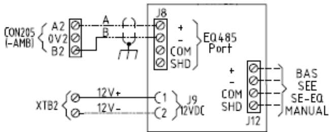
FIGURE 15 - SC-EQ CONNECTED IN YMAA, YVAE, AND YCWE
