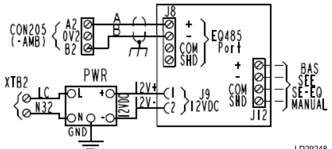
FIGURE 16 - SC-EQ CONNECTED IN YCAE AND YCWE-E
