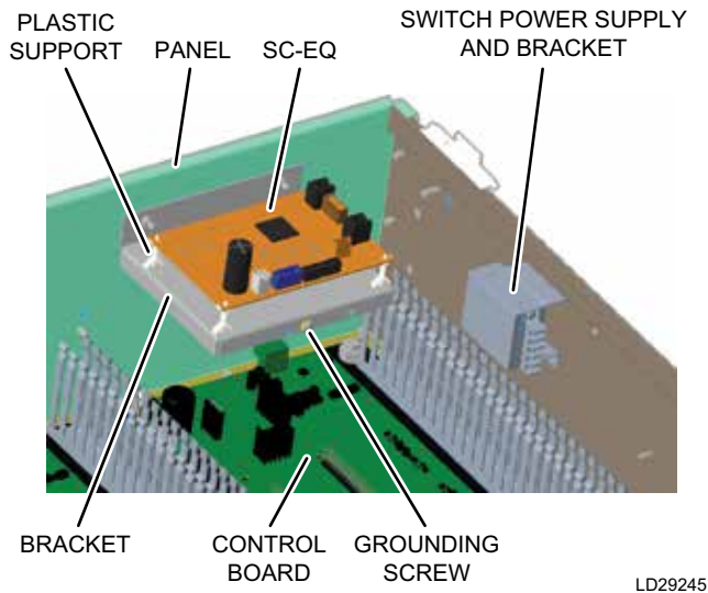
FIGURE 13 - SC-EQ INSTALLED IN YCAE
