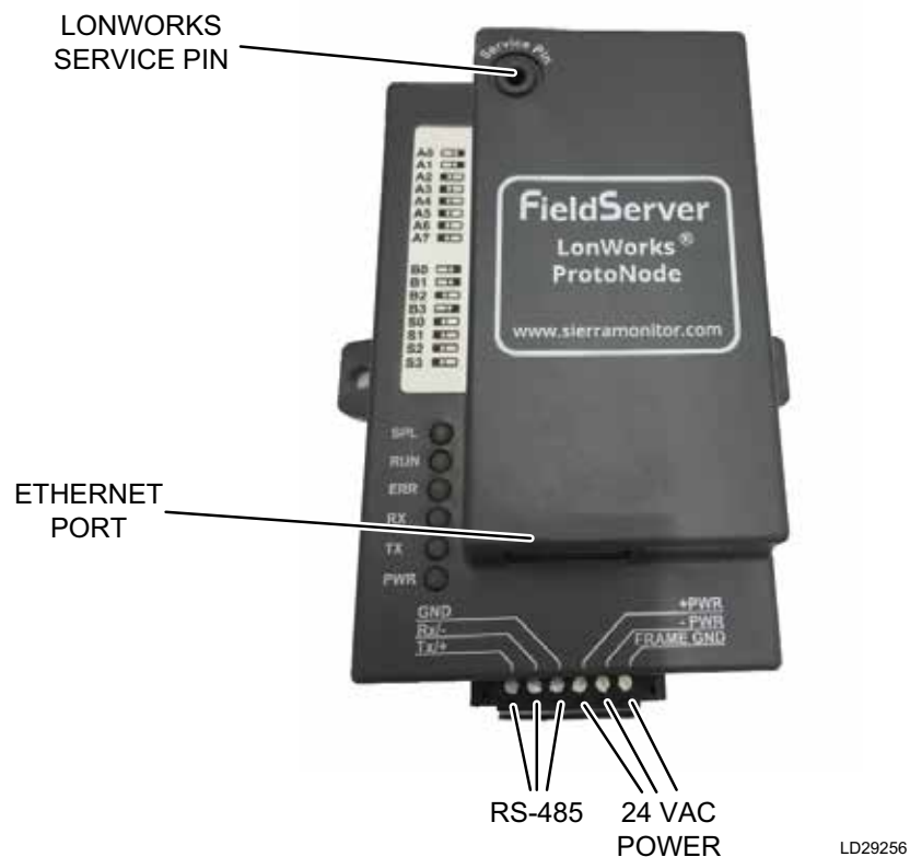
FIGURE 54 - LON PROTONODE FRONT VIEW
