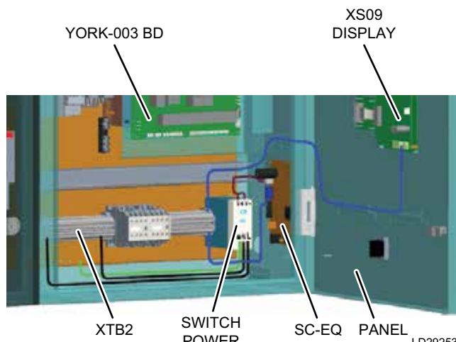
FIGURE 21 - SC-EQ INSTALLED IN YEW S TANDEM
