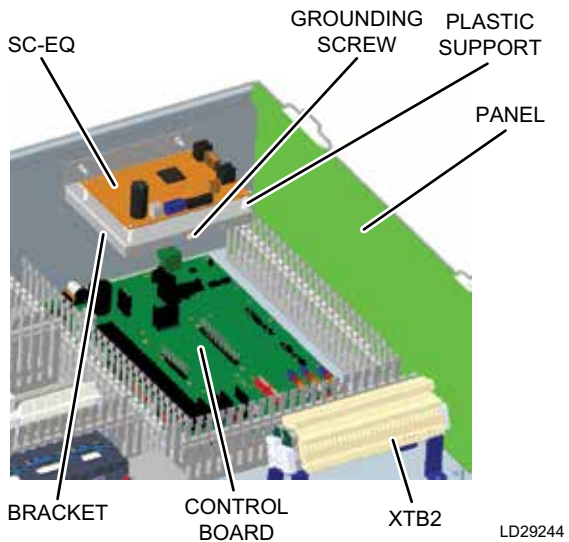
FIGURE 12 - SC-EQ INSTALLED IN YMAA AND YVAE
