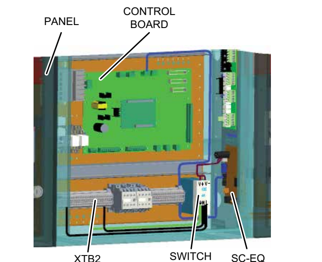
FIGURE 22 - SC-EQ INSTALLED IN YGWE TANDEM
