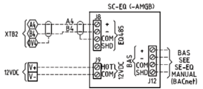
FIGURE 23 - SC-EQ TO YEW S CONNECTIONS
