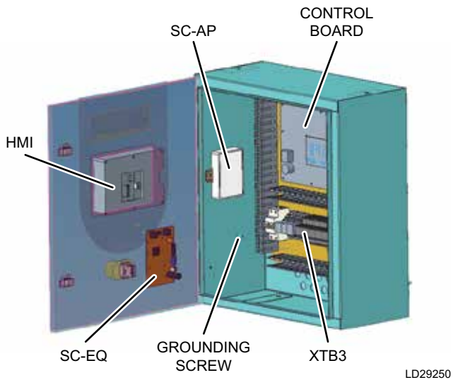
FIGURE 18 - SC-EQ INSTALLED IN YVWE AND YVWH
