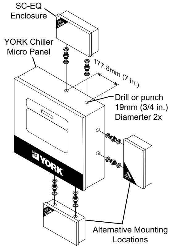
FIGURE 24 - MOUNTING ON THE EQUIPMENT
