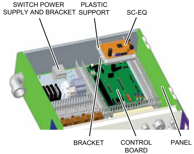
FIGURE 14 - SC-EQ INSTALLED IN YCWE-E
