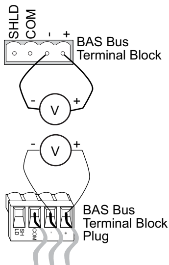
FIGURE 39 - BAS BUS METER CHECKS
