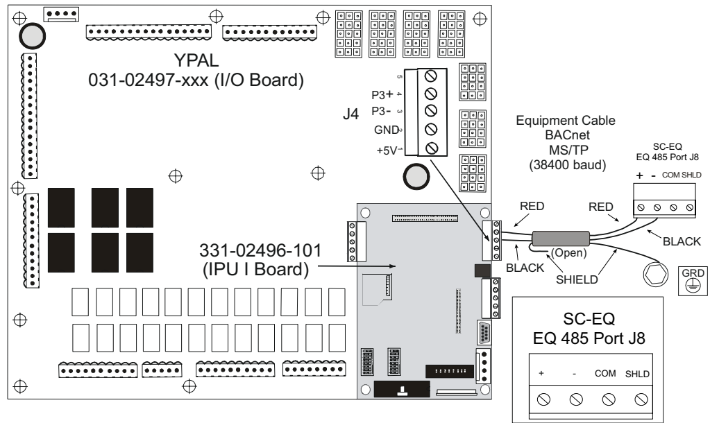
FIGURE 35 - SC-EQ COMM CARD CONNECTIONS FOR CHILLERS WITH THE 02550 MICROBOARD YCAL/YCUL/YLAA/YLPA/YCWL/YCRL/YSAA
