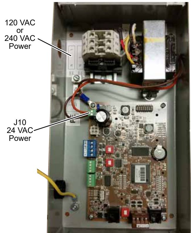
FIGURE 26 - SC-EQ IN ENCLOSURE
