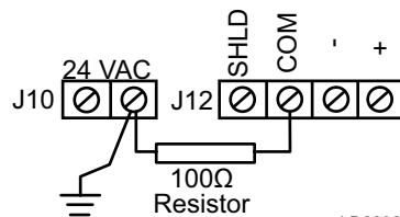
FIGURE 5 - 100 OHM RESISTOR INSTALLATION
