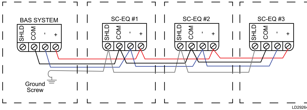
FIGURE 3 - 3-WIRE BAS
